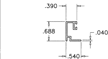
2 GLAZING BEAD
