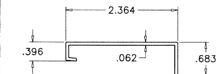
3 FRAME ADAPTER
